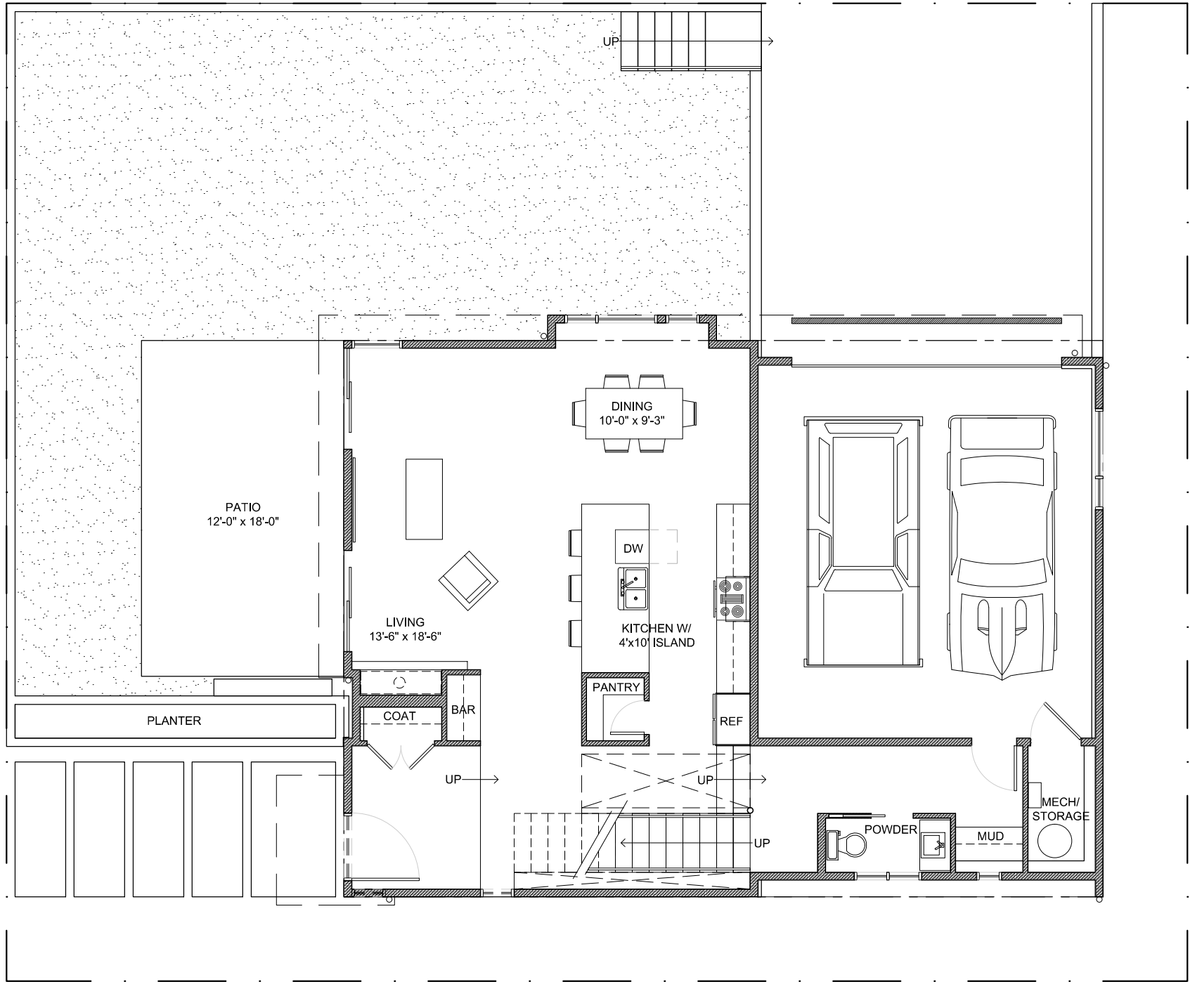
112TH AVE NE - NORTH UNIT | 1ST FLOOR PLAN
